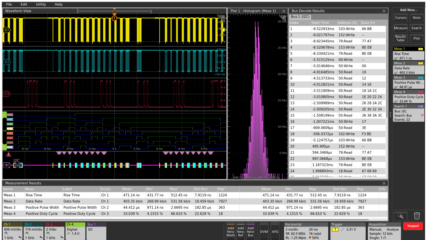
Viewing three analog channels, eight digital channels, a decoded serial bus waveform, decoded serial packet results table, four measurements, a measurement histogram, measurements results table with statistics and a search on serial bus events - simultaneously!
