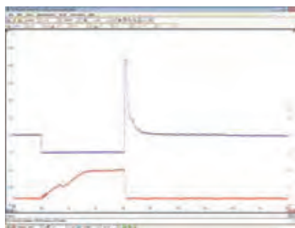
Petrol injectors
