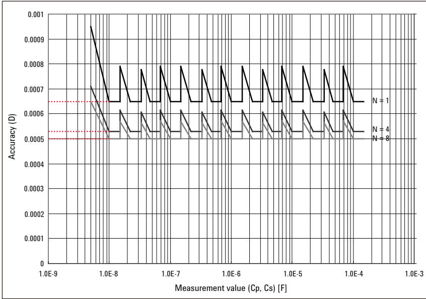
Figure 1. Accuracy of D when measurement frequency is 120 Hz (measurement range: 10 nF to 100 μF / measurement signal level: 0.5 V)
