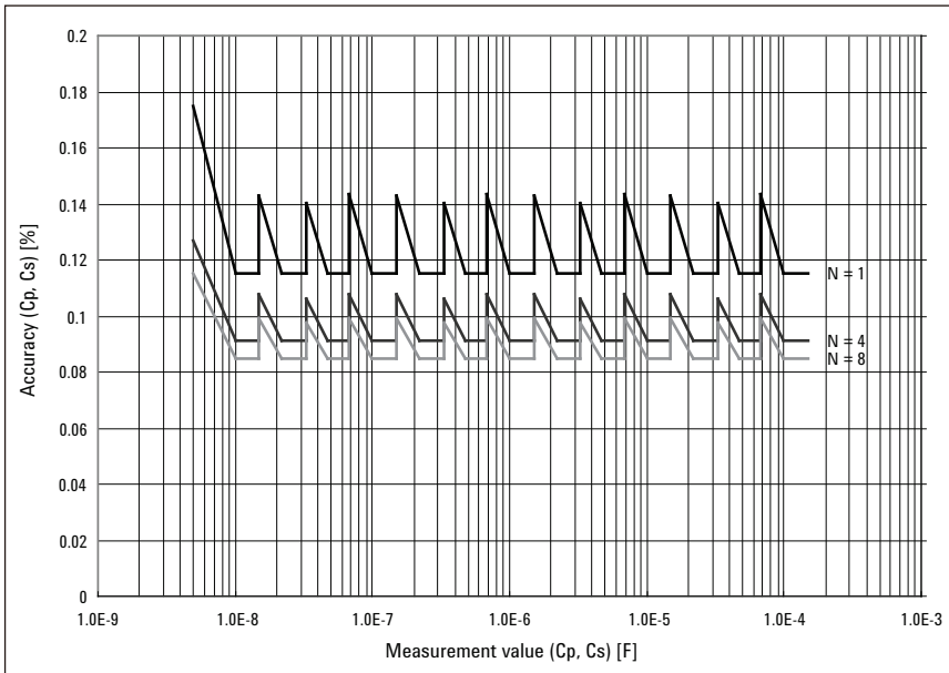
Figure 2. Accuracy of Cp and Cs when measurement frequency is 120 Hz (measurement range: 10 nF to 100 μF / measurement signal level: 0.5 V)
