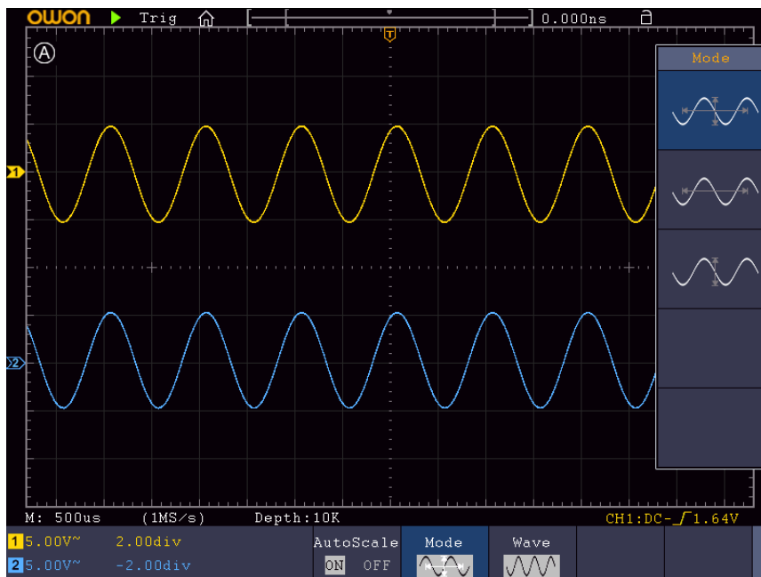
Figure 4-20 Autoscale Horizontal-Vertical multi-period waveforms
