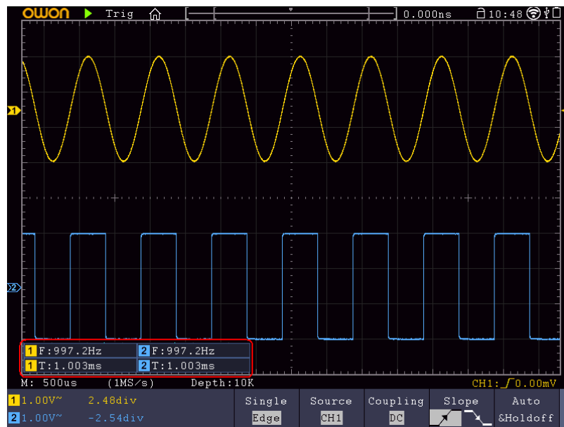
Figure 4-16 Automatic measurement
