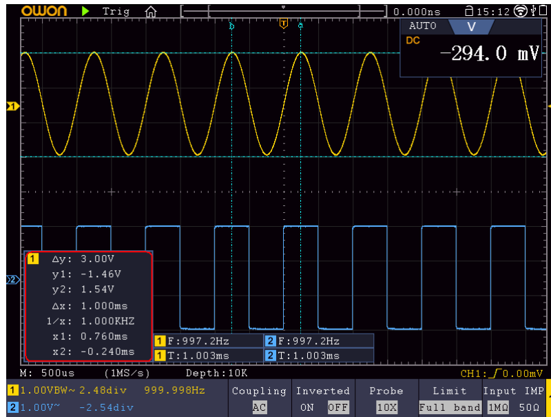
Figure 4-19 Time&Voltage Cursor Measurement
